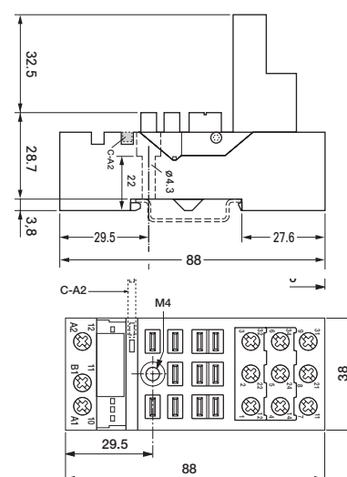
fig. 2. Dimension (mm)
